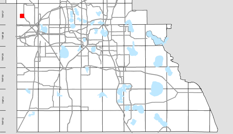
Location Map Polk County, Florida
